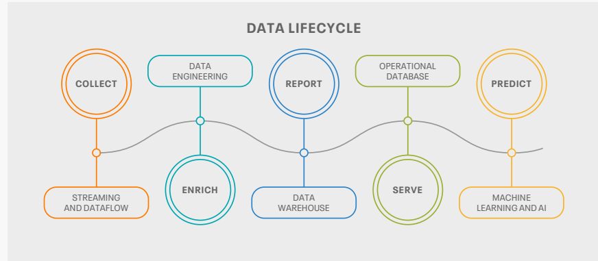
Image 2: Data Lifecycle
