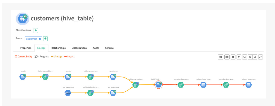
Image 6: Data Lineage
